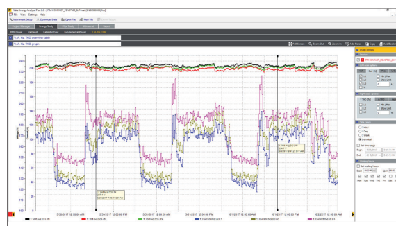
Voltage and current trend graph.
